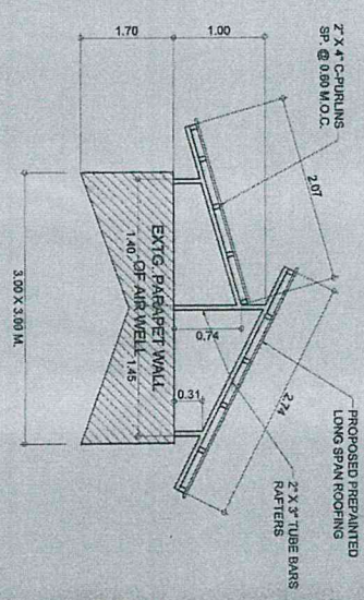
SECTION OF AIRWELL ROOFING SCALE: 1/100
